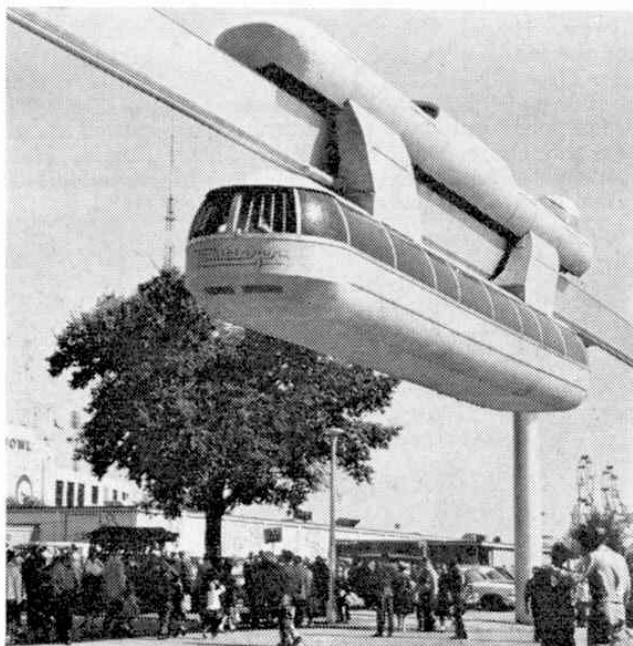
Above, the Safage monorail system as used at the United States World Fair. Here the cars are suspended from bogies. At left, another type of monorail, the U shaped hanger seen in Texas.
