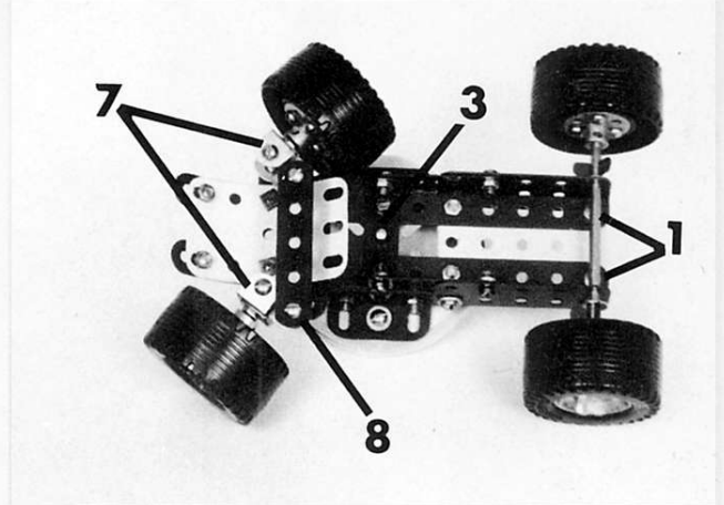
FIG. 3: The chassis as seen from below.
