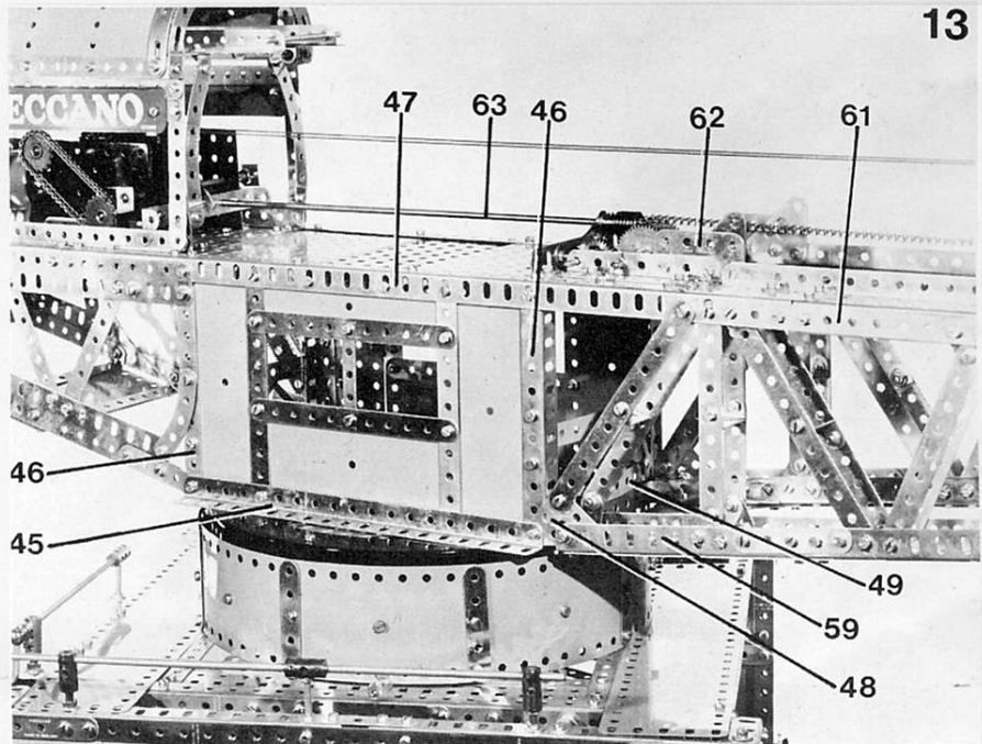
Fig. 13, a close-up view of the central portion of the boom secured to the upper turntable ring. Note that the boom is fixed to the ring at two points only, as described in the text. Construction of the control cabin representation is also fairly clear from this illustration.
