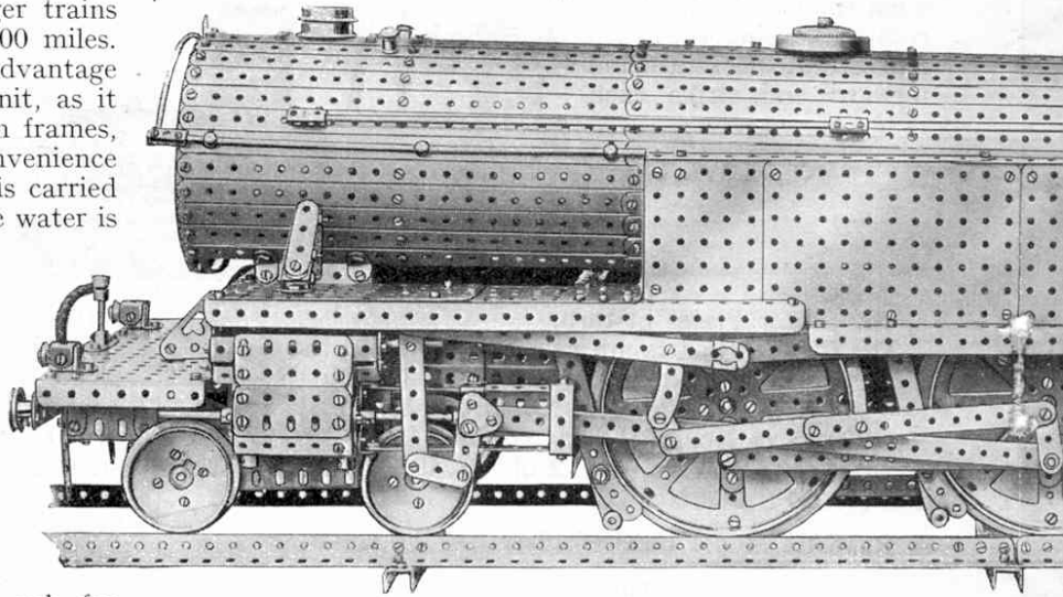
Fig. 2. General view of the Meccano model
