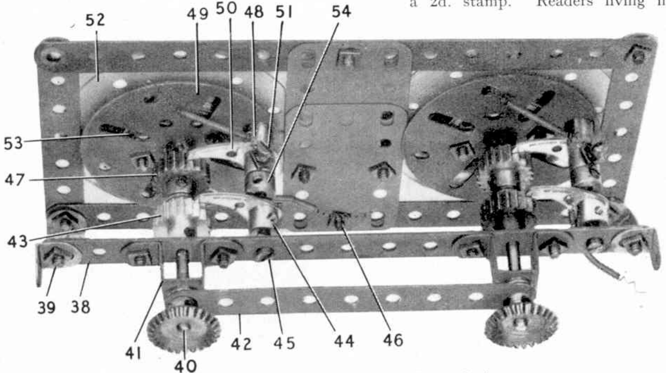
Fig. 2. An underneath view of the dialling mechanism.
