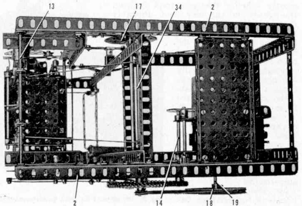
Fig. 2. An underneath view of the Cloth Folding Machine.
