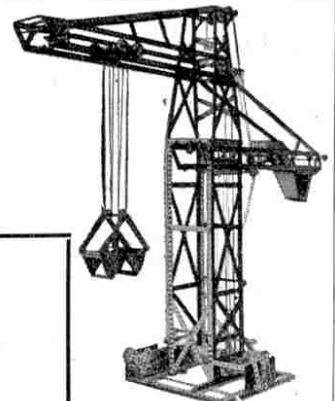
High-Speed Ship-Coaler
