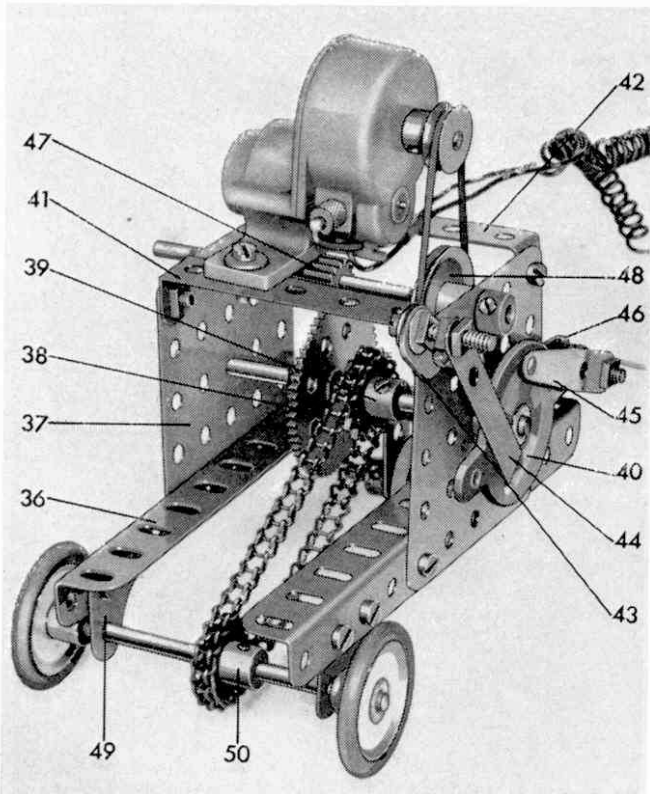
A view of the gearbox showing the drive and also the commutator arrangement.
