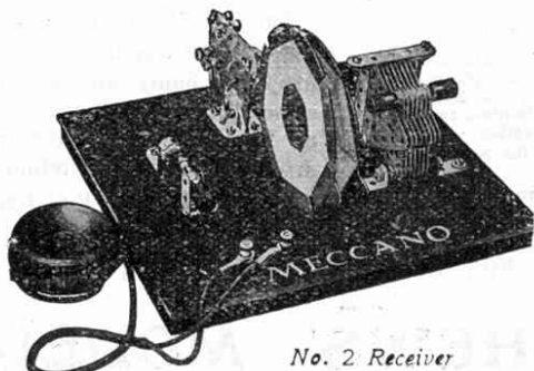
No. 2 Receiver
