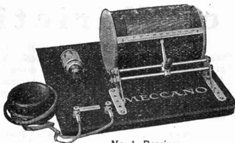
No. 1 Receiver
