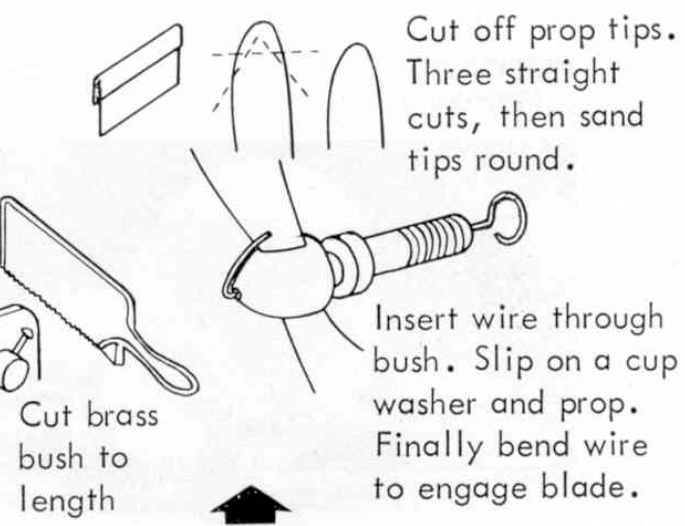
Assembly Stage 1
