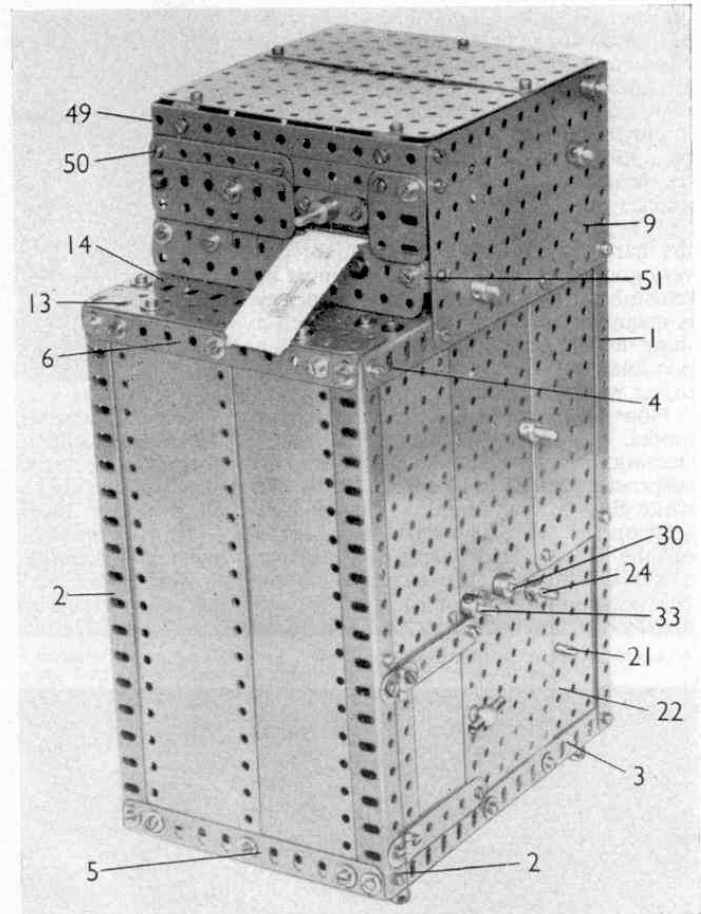
Fig. 1. The Automatic Ticket Machine in its completed state.
